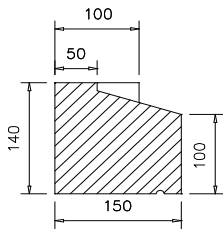
TYPE 4 CILL TYPICAL SECTION
