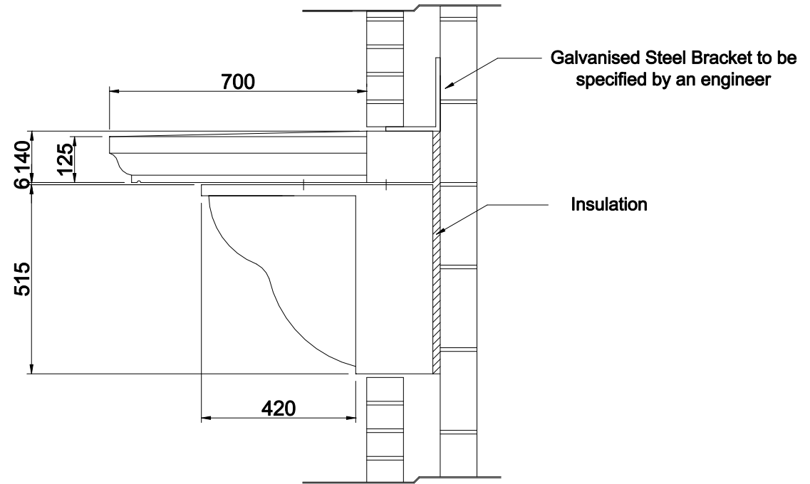
Side Elevation
