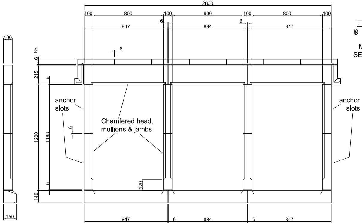
sectional view
