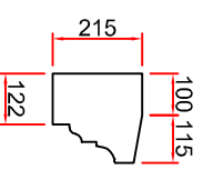
Head cornice section
