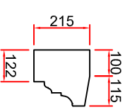
Head cornice section
