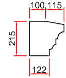
Head cornice section
